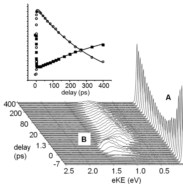
FIGURE 8. Time-resolved photoelectron spectrum of I^-(H_2O)_7 taken with pump and probe photon energies of 4.65 and 1.55 eV, respectively. 50 The inset illustrates the varying intensities of the transient feature (B) and the autodetachment signal (A).
