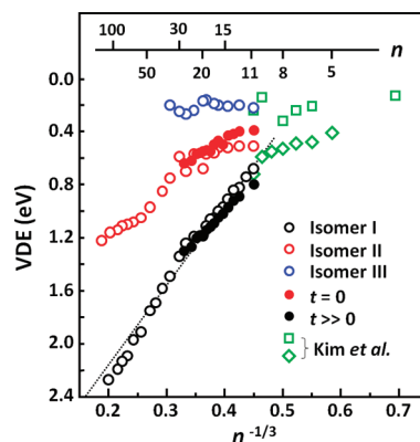
FIGURE 9. Size dependence of early ( t = 0 , filled red circles) and late ( t \gg 0 , filled black circles) VDEs of I^-(H_2O)_n following absorption in the CTTS band, along with VDEs of bare isomer I, II, and III water cluster anions.
